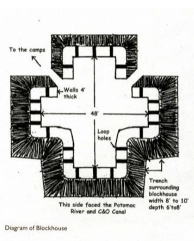
Blockhouse plan
